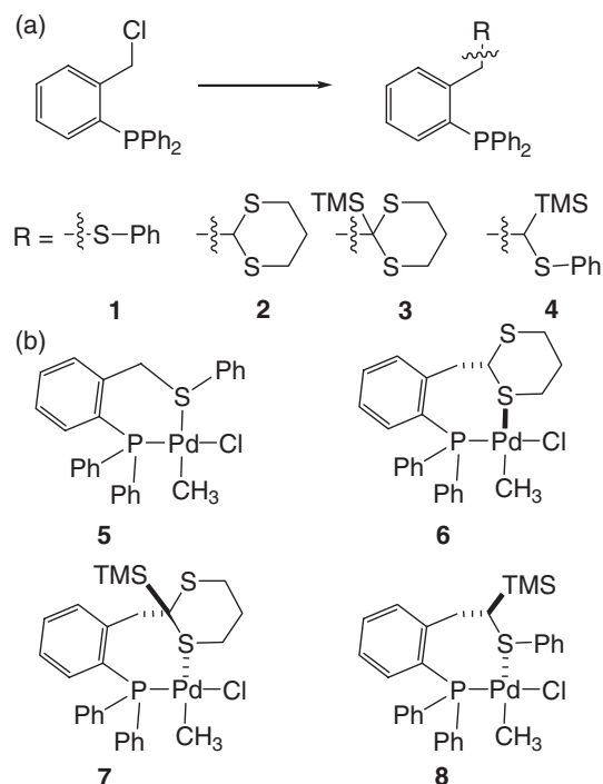
Figure 1. Phosphine–sulfide ligands 1–4 and Pd complexes 5–8 . The stereochemistry represents relative configuration but not absolute.
