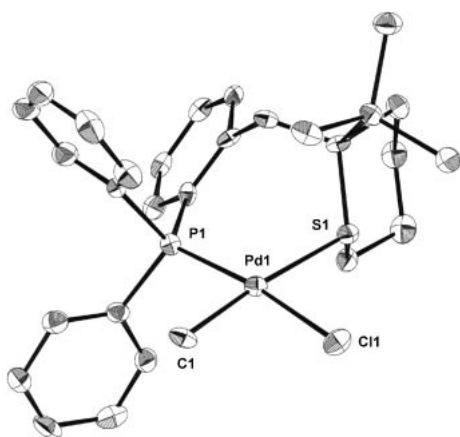
Figure 4. ORTEP drawing of 7 (all H atoms are omitted for clarity).
