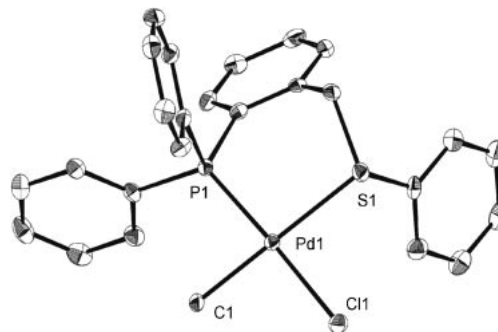
Figure 2. ORTEP drawing of 5 (all H atoms are omitted for clarity).
