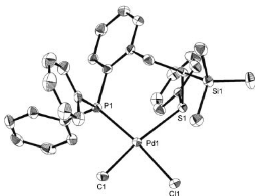
Figure 5. ORTEP drawing of 8 (all H atoms are omitted for clarity).
