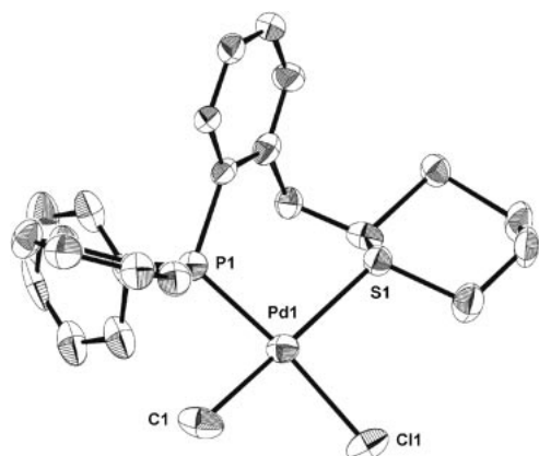
Figure 3. ORTEP drawing of 6 (all H atoms are omitted for clarity).
